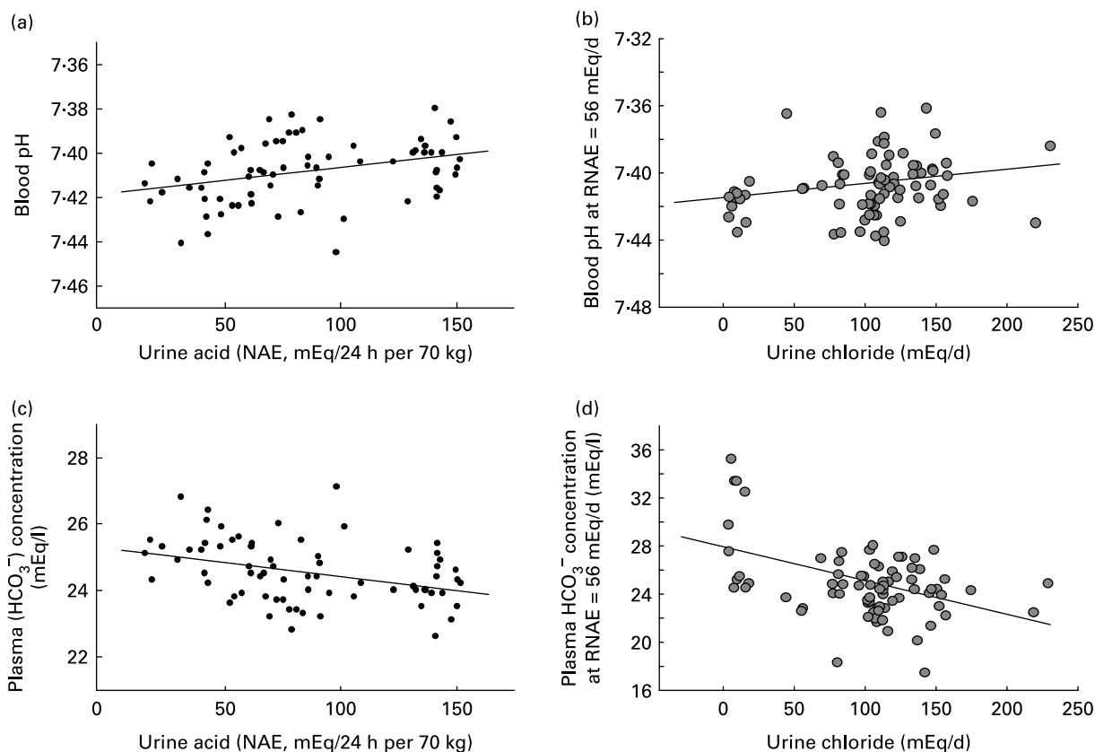
Fig. 1. (a) Blood pH at constant net acid excretion (NAE) rate ( r = 0.34 ; P < 0.005 ). (b) Blood pH at constant urinary chloride excretion rate (renal NAE (RNAE) = 56 \text{ mEq/d} ) ( r = 0.22 ; P < 0.05 ). (c) Plasma bicarbonate at constant NAE rate ( r = -0.36 ; P < 0.005 ). (d) Plasma bicarbonate at constant urinary chloride excretion rate (RNAE = 56 \text{ mEq/d} ) ( r = -0.45 ; P < 0.001 ). Adapted from Frassetto et al. (6) .
